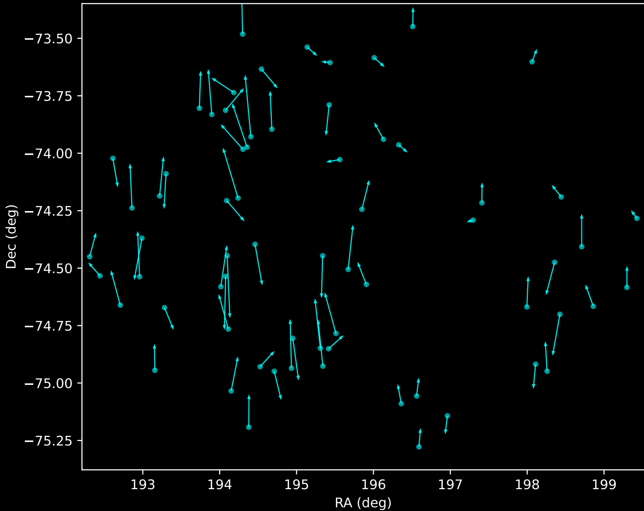
GALAH DR4 Noise Stream Proper Motion Vectors (n=67)
