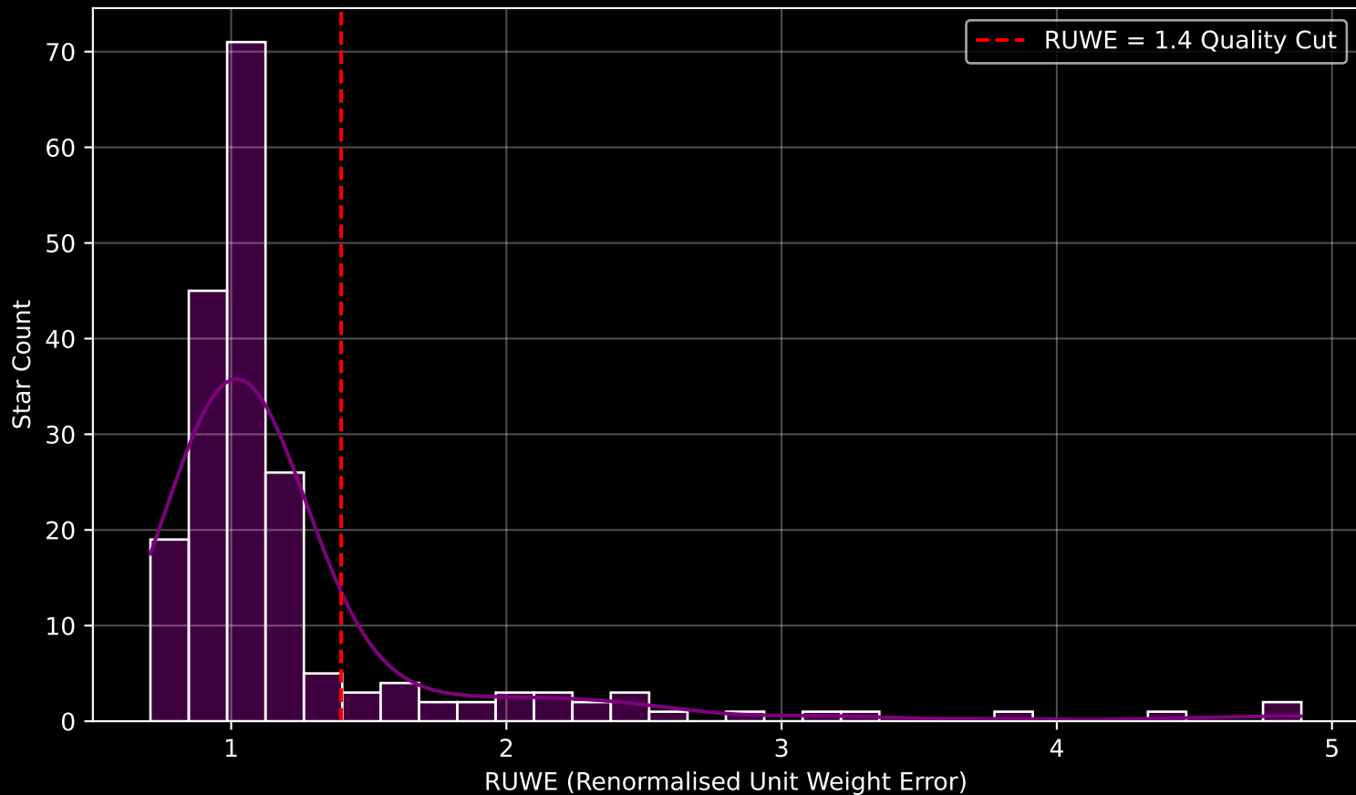
GALAH DR4 Field [7172] RUWE Distribution (n= 196)
