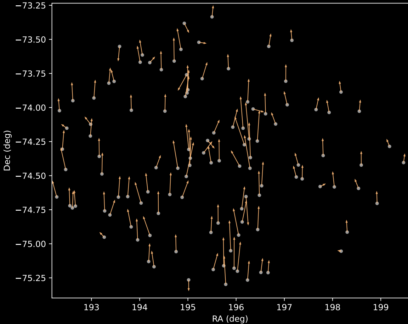
GALAH DR4 Cluster 3 Proper Motion Vectors (n=113)
