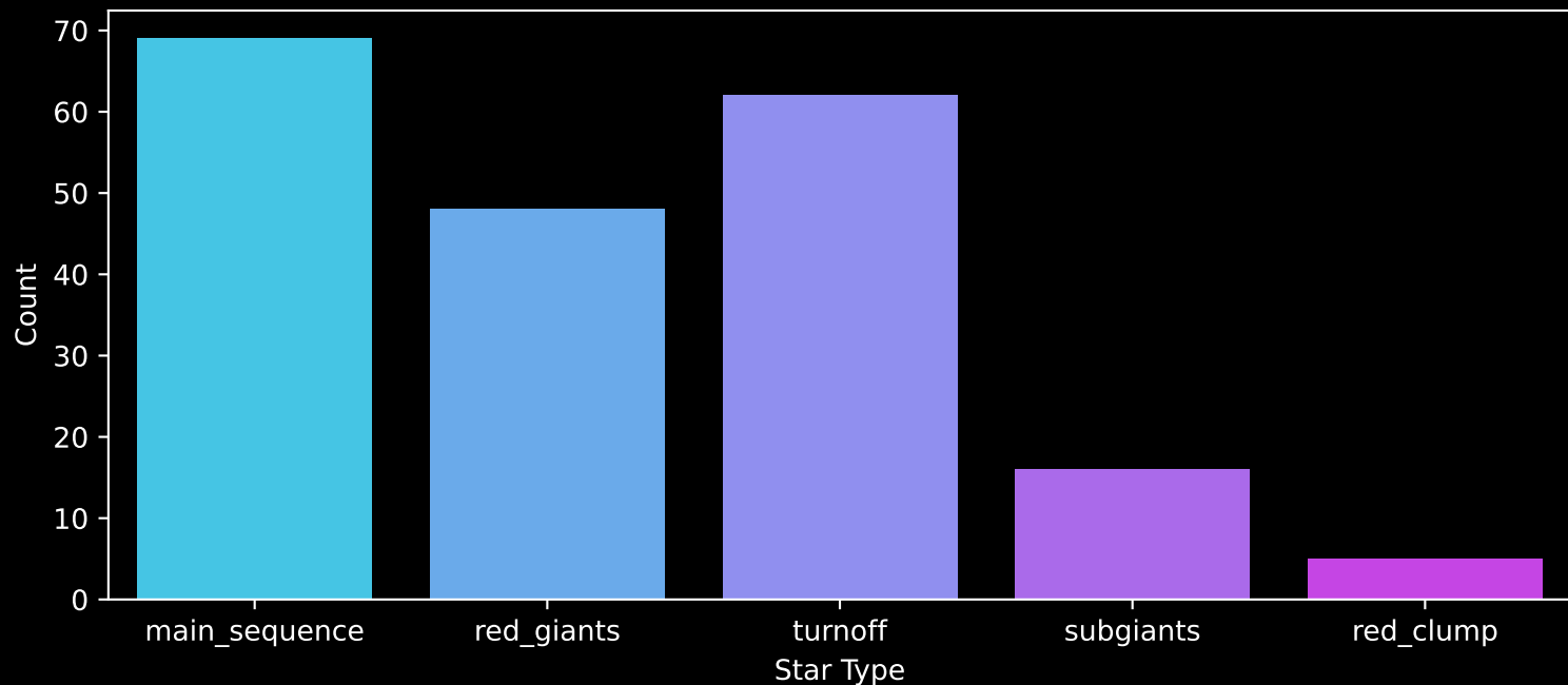
GALAH DR4 Field: [7172] Count plot of Star Type
