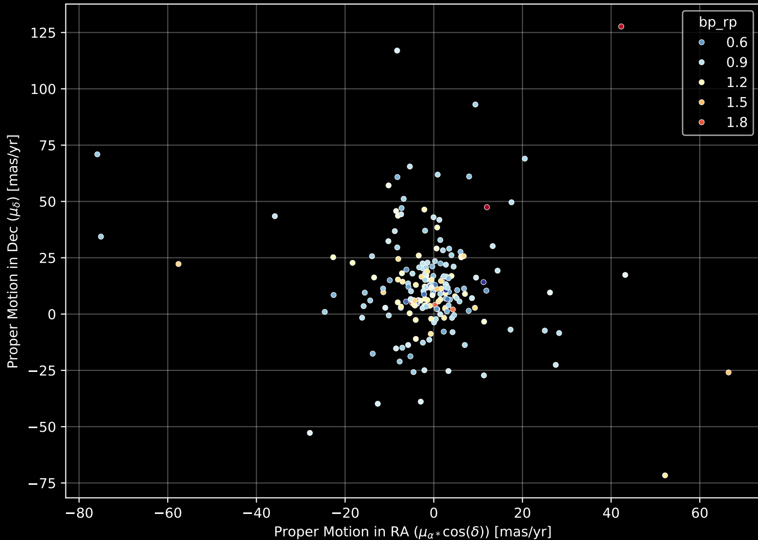
GALAH DR4 Field: [7172] Proper Motion Diagram (n= 200)
